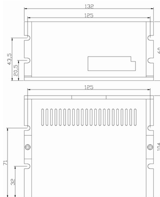
Figure 1: Mechanical specifications
