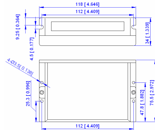
Figure 1: Mechanical specifications
