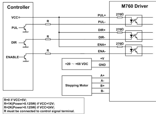
Figure 10: Typical connection
